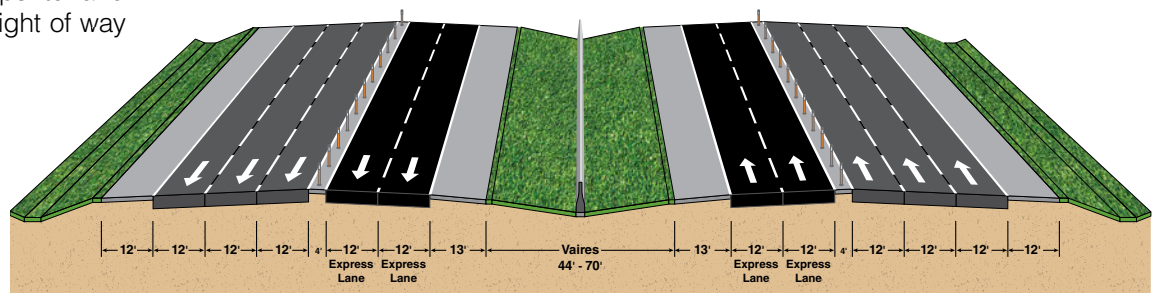
Buffer Separated Express Lanes with Preserved Transit Corridor (Design Accommodates Potential Future Rail)
